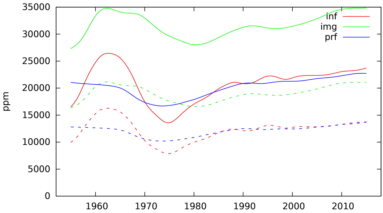
lemma_byt'
