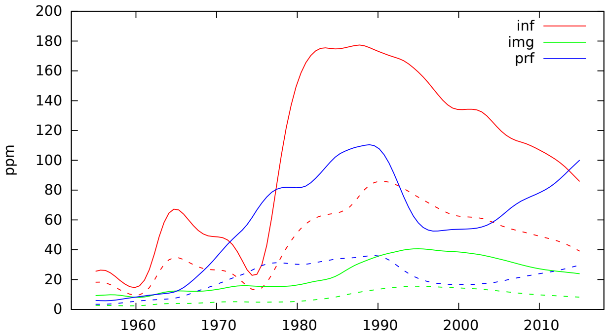
lemma_televizny
