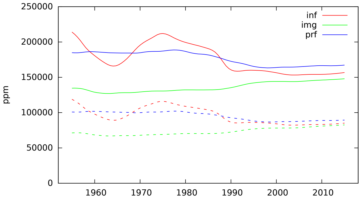
gender_f
