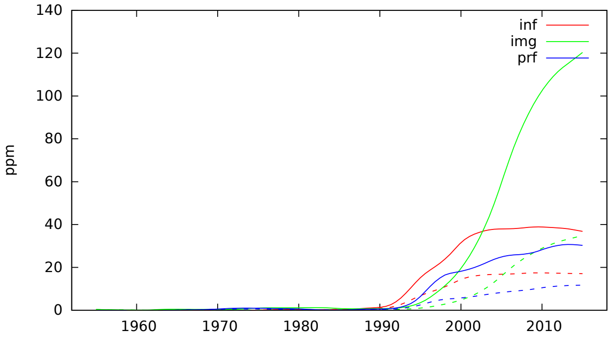
lemma_mobil
