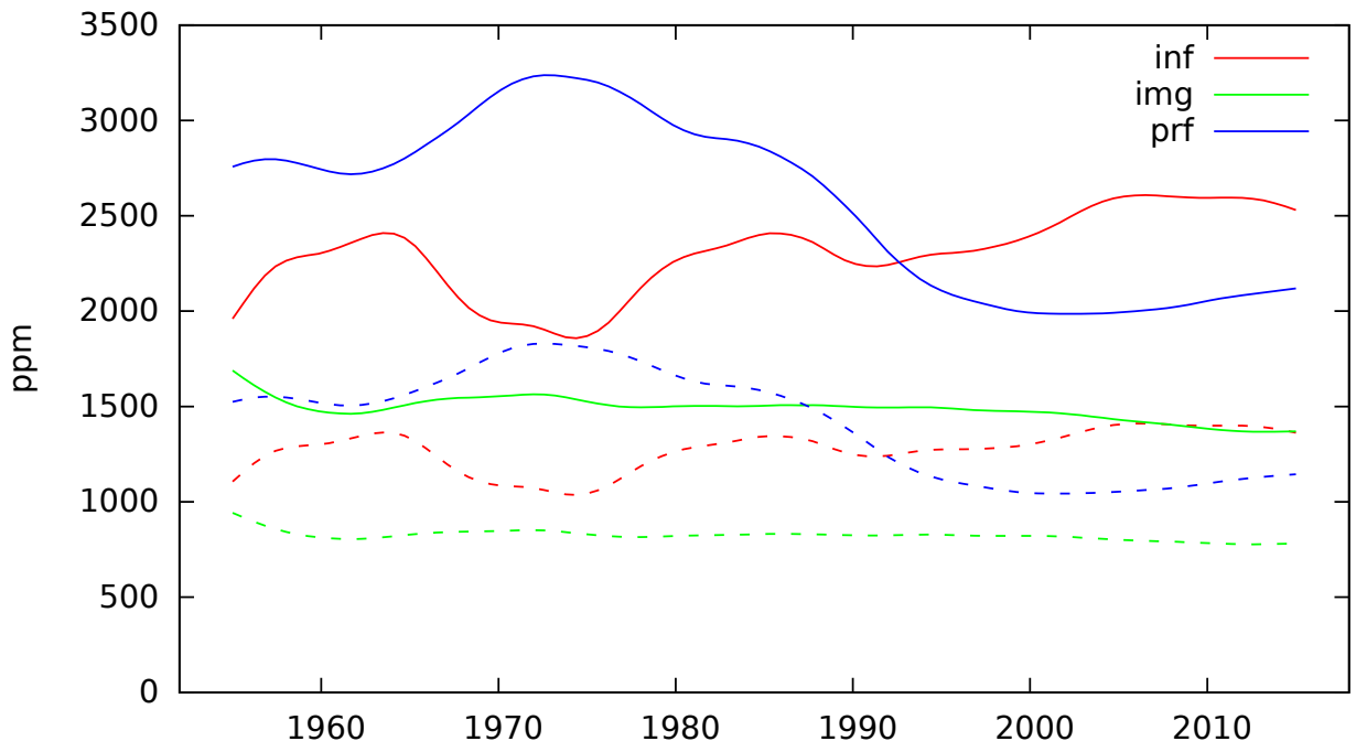
degree_z
