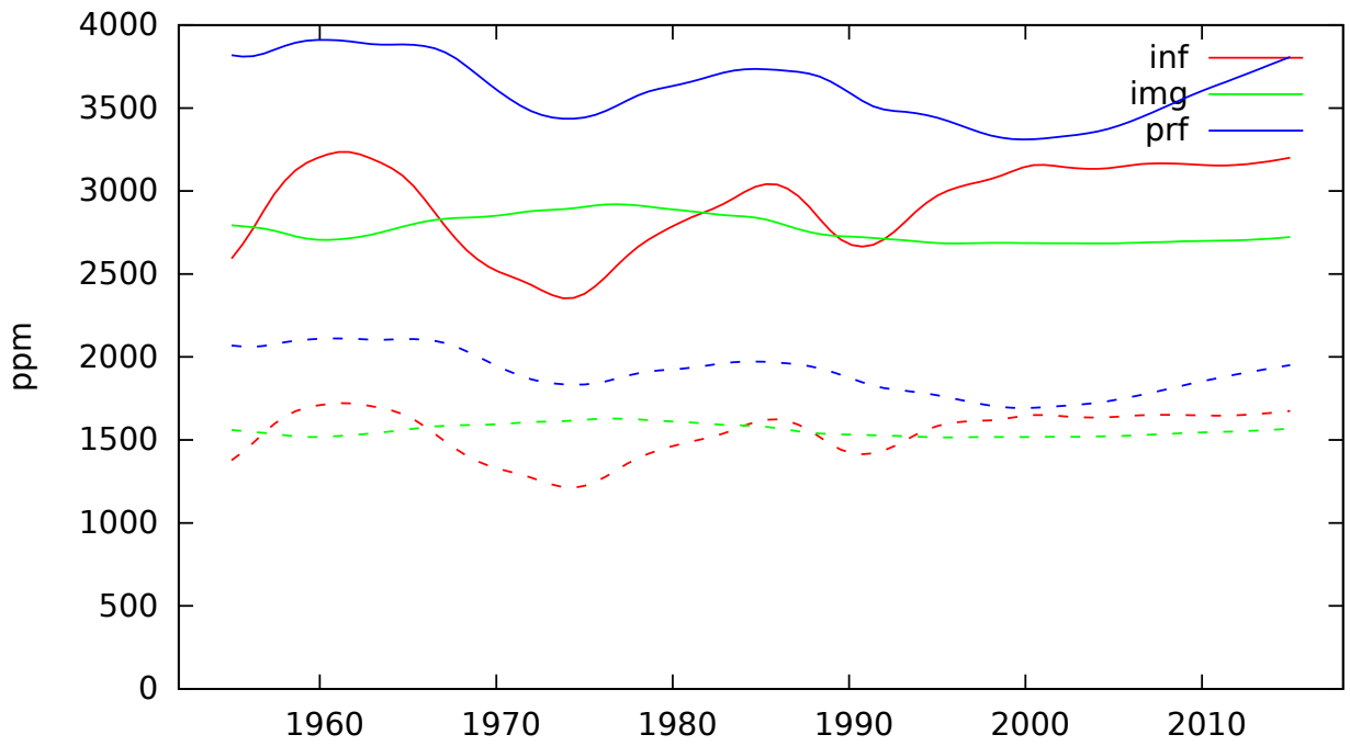
degree_y
