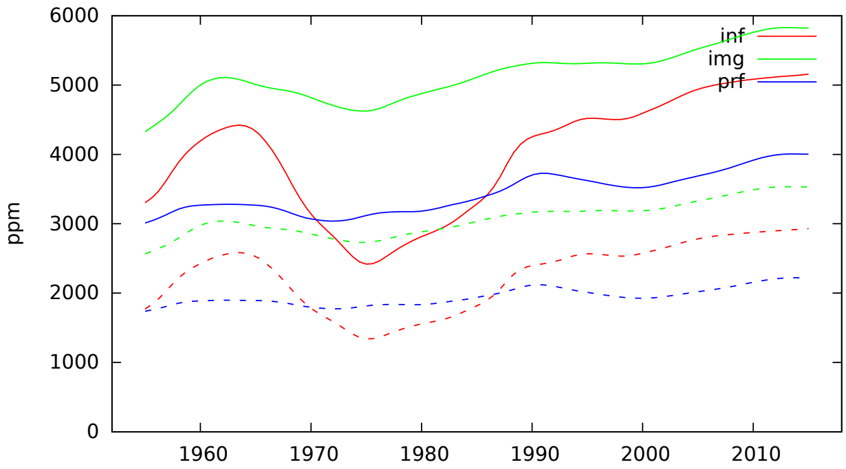
lemma_mat'
